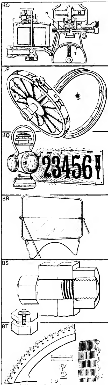
BO—Section through the Homo type of carbureter BP—Denegre demountable rim and wheel felloe BQ—Gus Balzer tail lamp for license number plates BR—Vision automatic windshield without metal division BS—Columbia nut on bolt and improved form of nut BT—Link-Belt silent chain and details of construction
